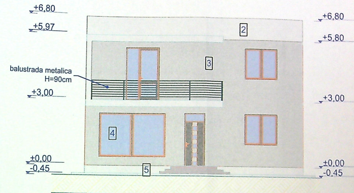
FATADA PRINCIPALA scara 1:100
