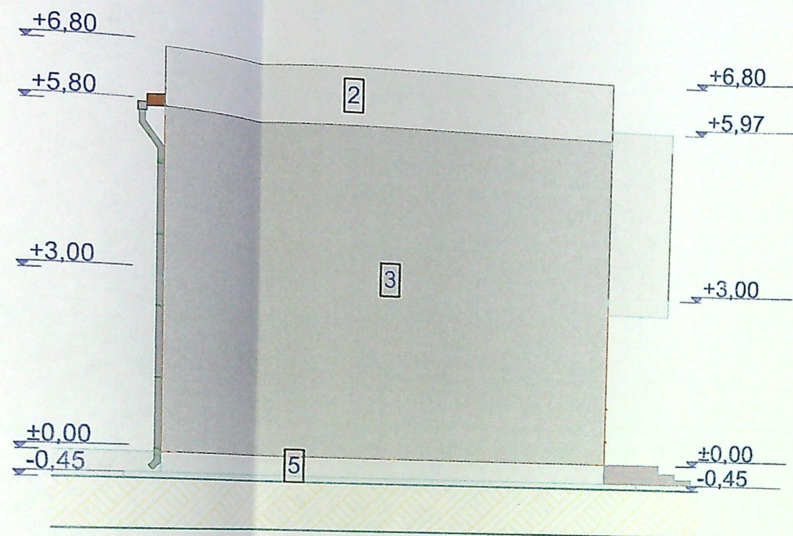
FATADA STANGA scara 1:100
